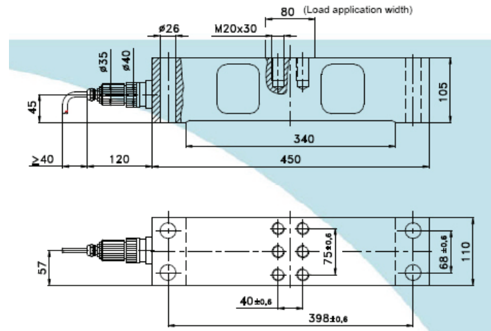
DWB 40t
