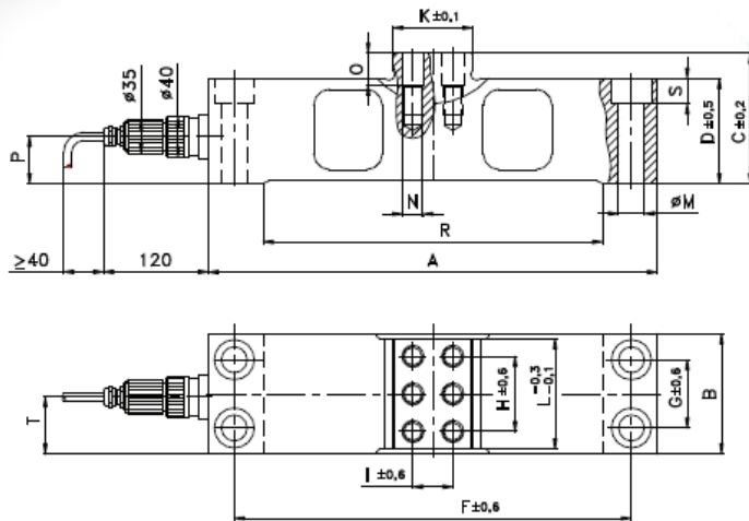
DWB 50-200t
